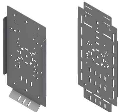
Typical standard Equipment plates.
